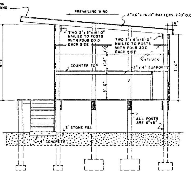
SECTION X-X
