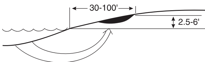
Figure 2a. Saline soil development near shallow streams, road ditches and sewage lagoons.
