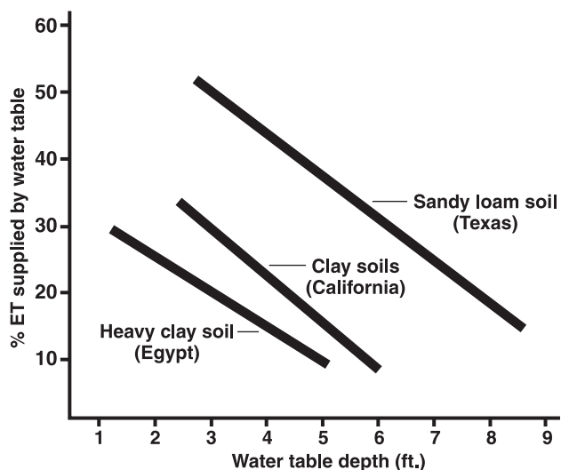
Figure 7. Evapotranspiration supplied by a saline water table as affected by water table depth. (Gismer and Gates, 1988).
