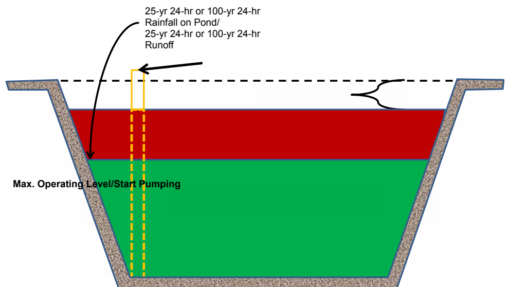
Fig. 1. Capacity of a runoff storage pond (not to scale).
