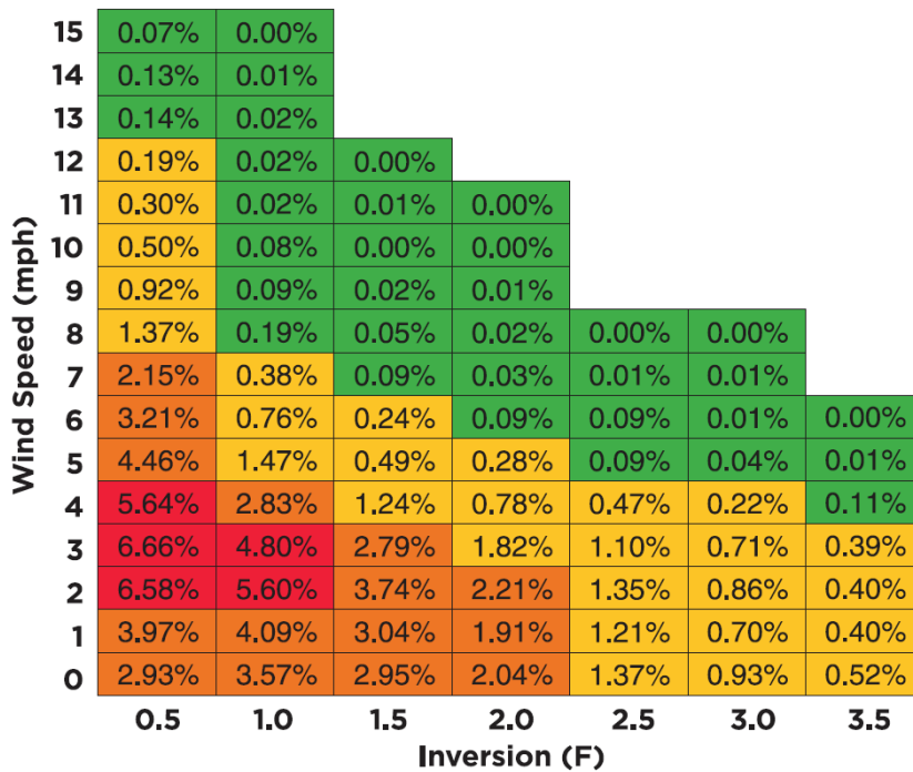
Significant inversion conditions can exist in wind speeds of 6 mph or more. This chart shows the percent of time that several NDAWN stations indicated an air temperature inversion. For example, 4.80% of the time an inversion of 1 degree existed with a 3 mph breeze.
