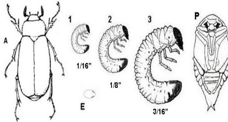
Life stages of Phyllophaga implicita : A - adult June beetle; E - egg; grub stages with their head width in inches, 1 - first; 2 - second; 3 - third; and P - pupa.
