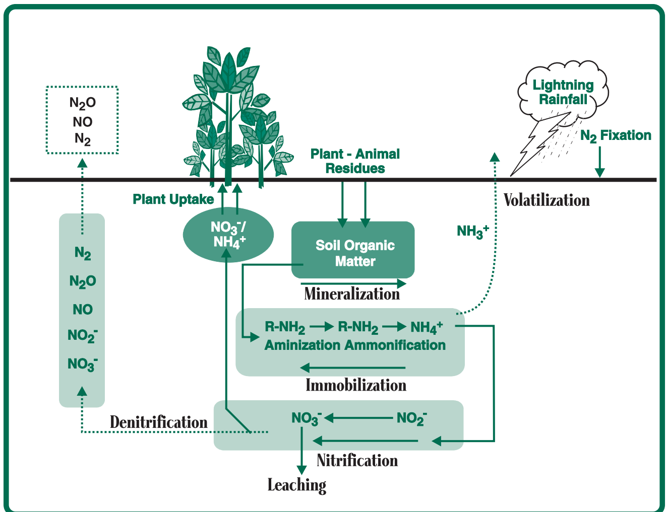
Figure 1. The nitrogen cycle. (Source: Livestock and Poultry Environmental Stewardship Curriculum)
