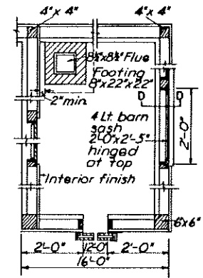
PLAN OF SHOP
