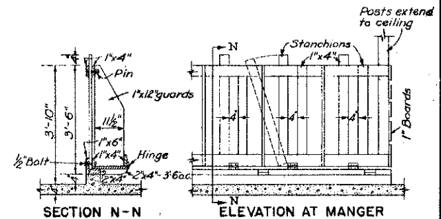
FALSE FLOOR CALF PEN TO BE USED IN BOX STALL
