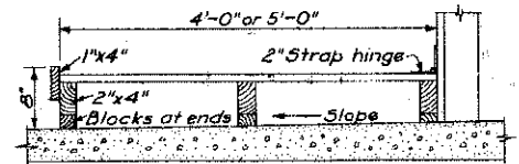
SECTION M-M
