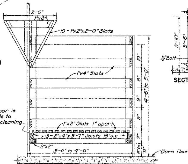
FALSE FLOOR CALF PEN TO BE USED IN BOX STALL
