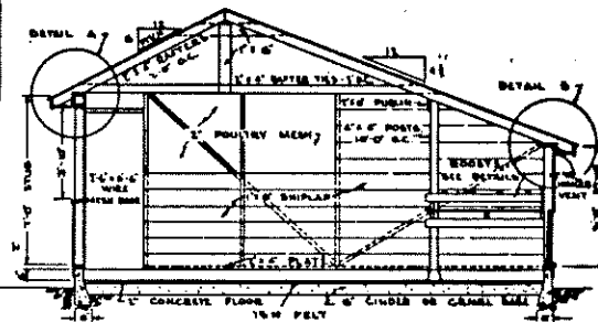
CROSS SECTION - COMBINATION ROOF
