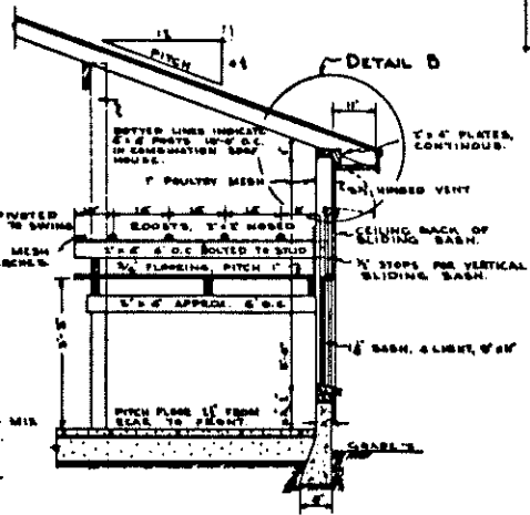
TYPICAL WALL SECTIONS
