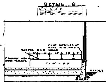
ALTERNATE ROOST DETAIL
