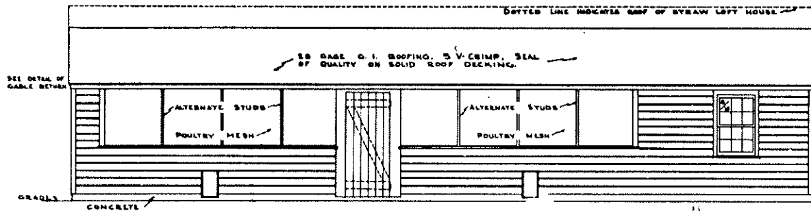
FRONT ELEVATION COMBINATION ROOF & STRAW LOFT TYPES
