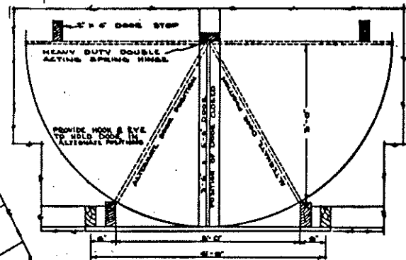
DETAIL OF DOUBLE ACTION DOOR
