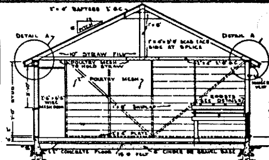
CROSS SECTION - STRAW LOFT TYPE
