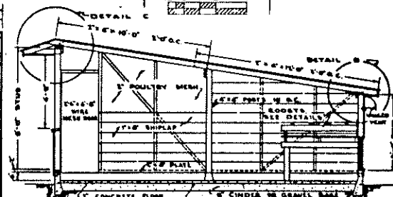
CROSS SECTION - SHED ROOF
