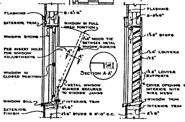
• WINDOW SECTION •
