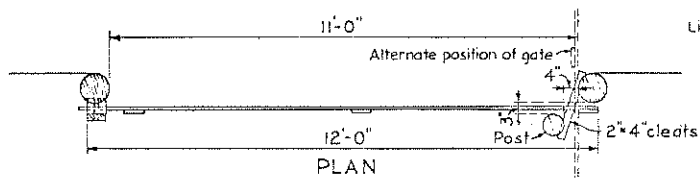
LIFT GATE TYPE-B
