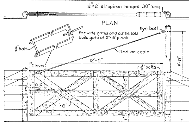
Block 18" long bolted to post TYPE-D
