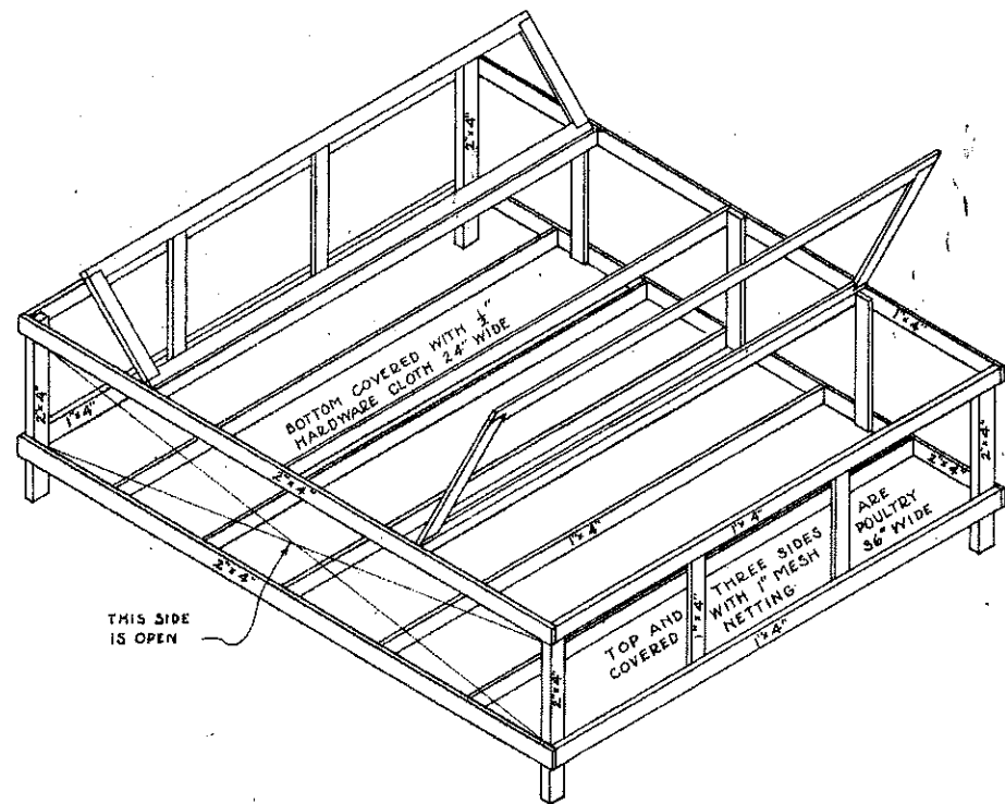
ISOMETRIC VIEW SCALE \frac{1}{2} "=1'-0"
