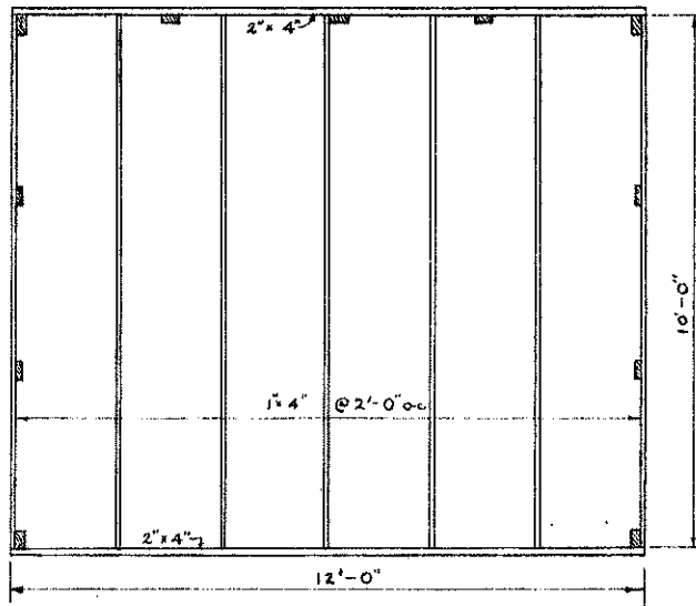
PLAN OF BOTTOM SCALE \frac{1}{2} "=1'-0"
