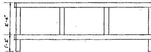
SIDE ELEVATION SCALE \frac{1}{2} "=1'-0"
