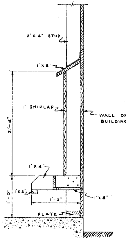
SECTION SCALE 1\frac{1}{2}'' = 1'-0''
