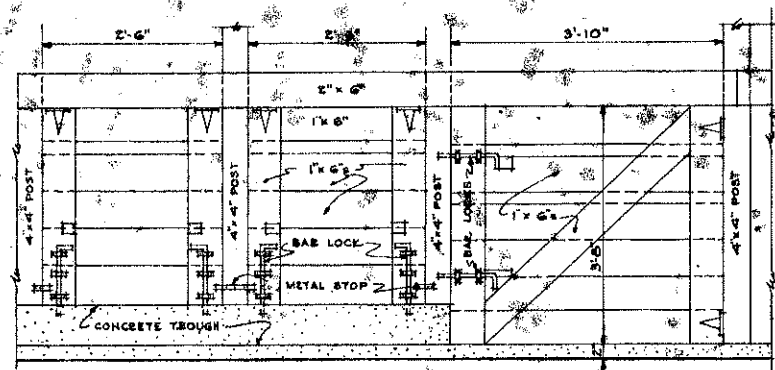
ELEVATION OF PEN GATES AND TROUGHS SCALE: \frac{3}{4} " = 1'-0"
