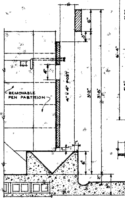
CONCRETE TROUGH WITH SOLID FRONT PANEL
