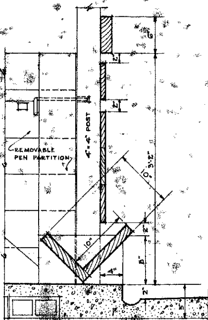
REMOVABLE WOOD TROUGH WITH SOLID FRONT PANEL
