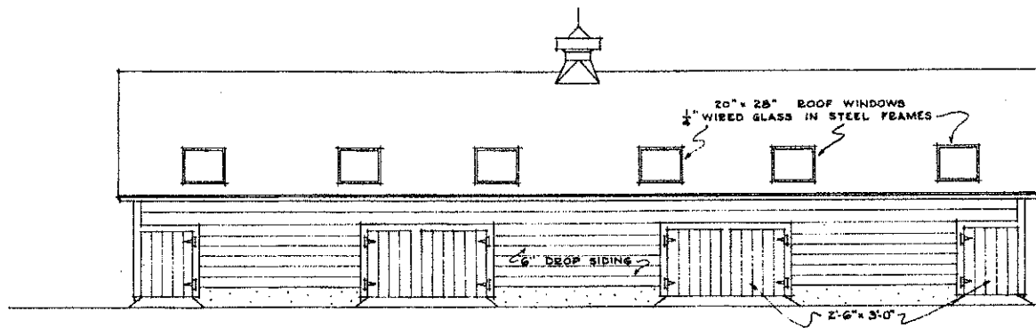
SOUTH ELEVATION SCALE \frac{1}{4} " = 1'-0"
