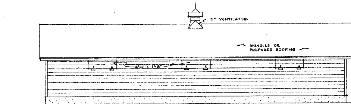
NORTH ELEVATION SCALE \frac{1}{4} " = 1'-0"
