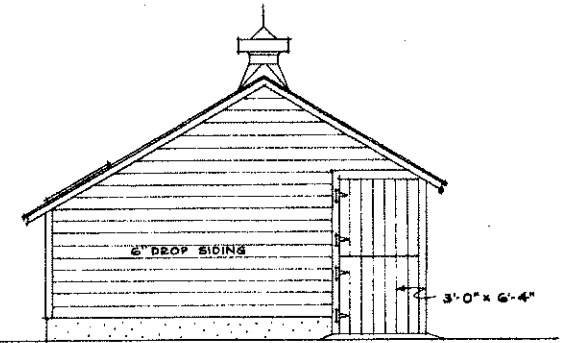
EAST ELEVATION SCALE \frac{1}{4} " = 1'-0"
