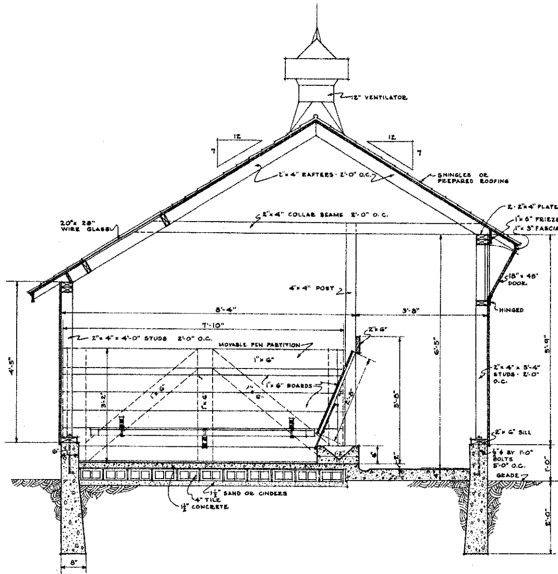
SECTION SCALE \frac{1}{2} " = 1'-0"
