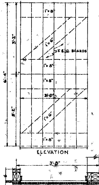
JAMB SECTION DETAIL OF DOORS IN EAST & WEST WALLS SCALE: \frac{3}{4} " = 1'-0"
