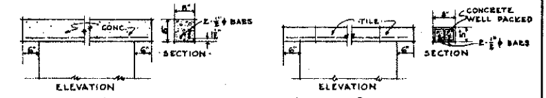
LINTEL DETAIL FOR BRICK OR CONCRETE BLOCK WALL SCALE \frac{1}{2} " = 1'-0"
