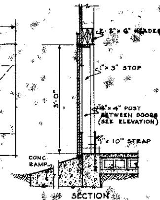
SECTION DETAIL OF DOORS IN SOUTH WALL SCALE: \frac{3}{4} " = 1'-0"
