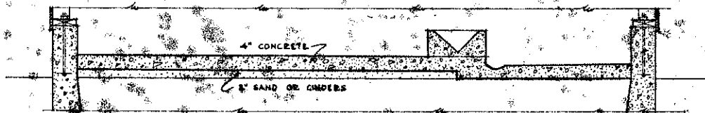
SECTION THRU ALTERNATE FLOOR CONSTRUCTION SCALE: \frac{3}{4} " = 1'-0"
