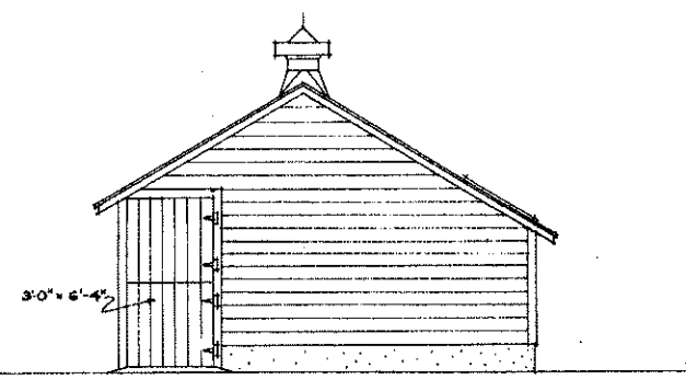
WEST ELEVATION SCALE \frac{1}{4} " = 1'-0"
