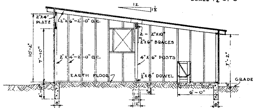
CROSS SECTION SCALE \frac{1}{4}'' = 1'-0''
