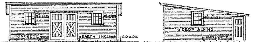
FRONT ELEVATION [SOUTH] SCALE \frac{1}{8}'' = 1'-0''
