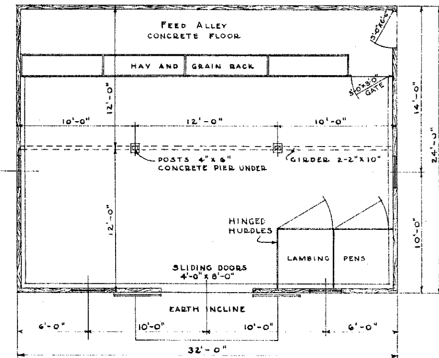
PLAN SCALE \frac{1}{4}'' = 1'-0''
