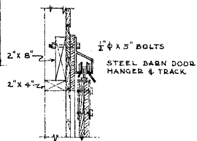
SLIDING DOOR DETAILS SCALE 1\frac{1}{2}'' = 1'-0''
