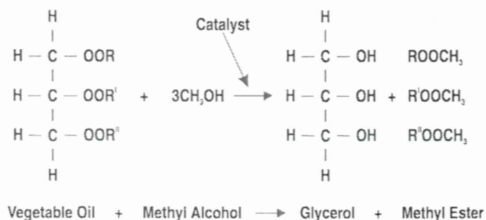
Figure 2. Transesterification of vegetable oils.
