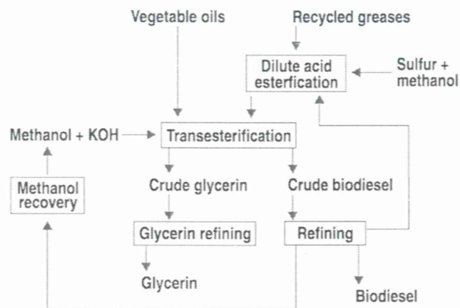
Figure 1. Basic transesterification technology.
