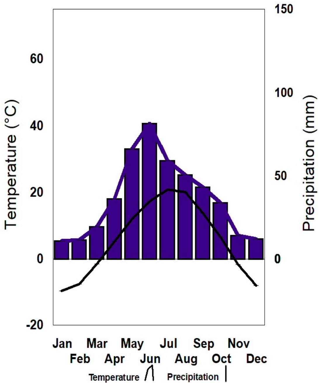
Figure 2. Ombrothermic diagram of long-term mean monthly temperature and monthly precipitation at the DREC Ranch, western North Dakota, 1982-2019.
