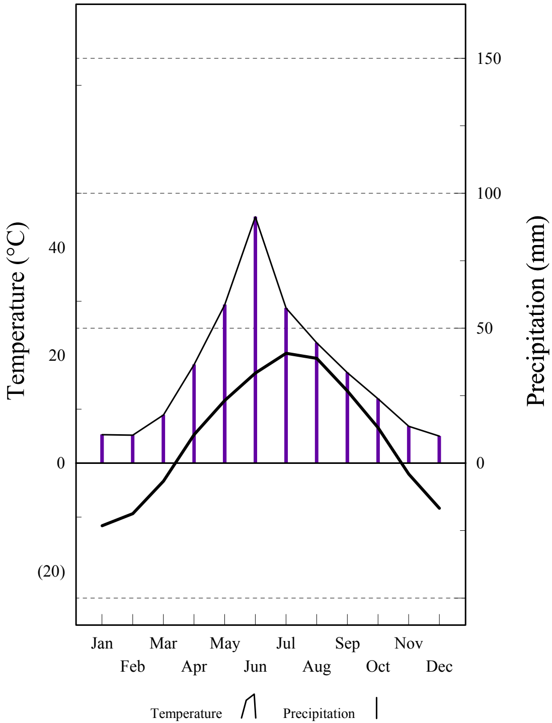
Fig. 2. Ombrothermic diagram of long-term (1892-2002) mean monthly temperature and monthly precipitation at Dickinson, North Dakota.
