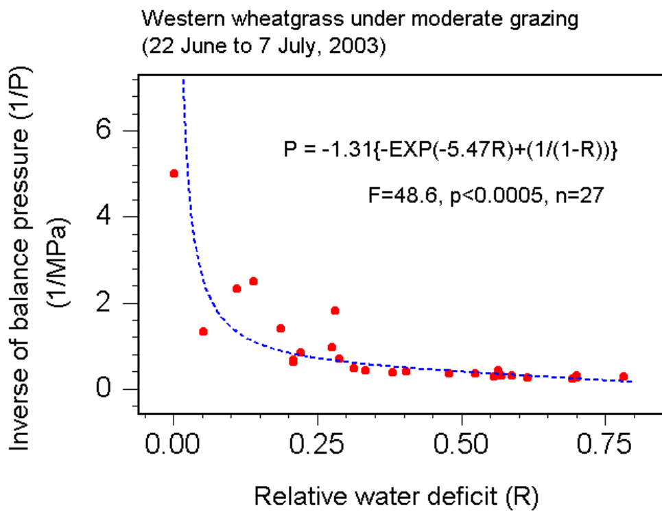
Figure 7: A sample pressure-volume curve for plant leaf.
