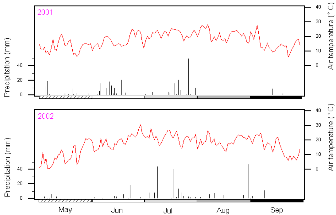
Figure 2: Daily precipitation and temperature in the growing season of 2001 and 2002. Note that 2001 had a dry late summer and 2002 had a dry spring.
