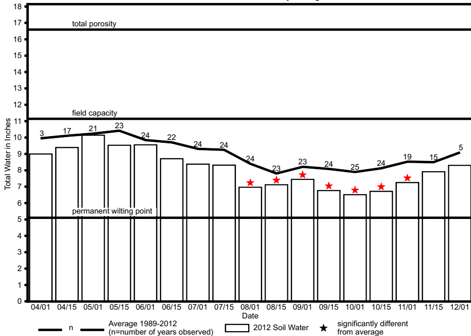
Total water in soil profile to the two and one half foot depth on loamy ecological sites at the Central Grasslands Research Extension Center in 2012.
