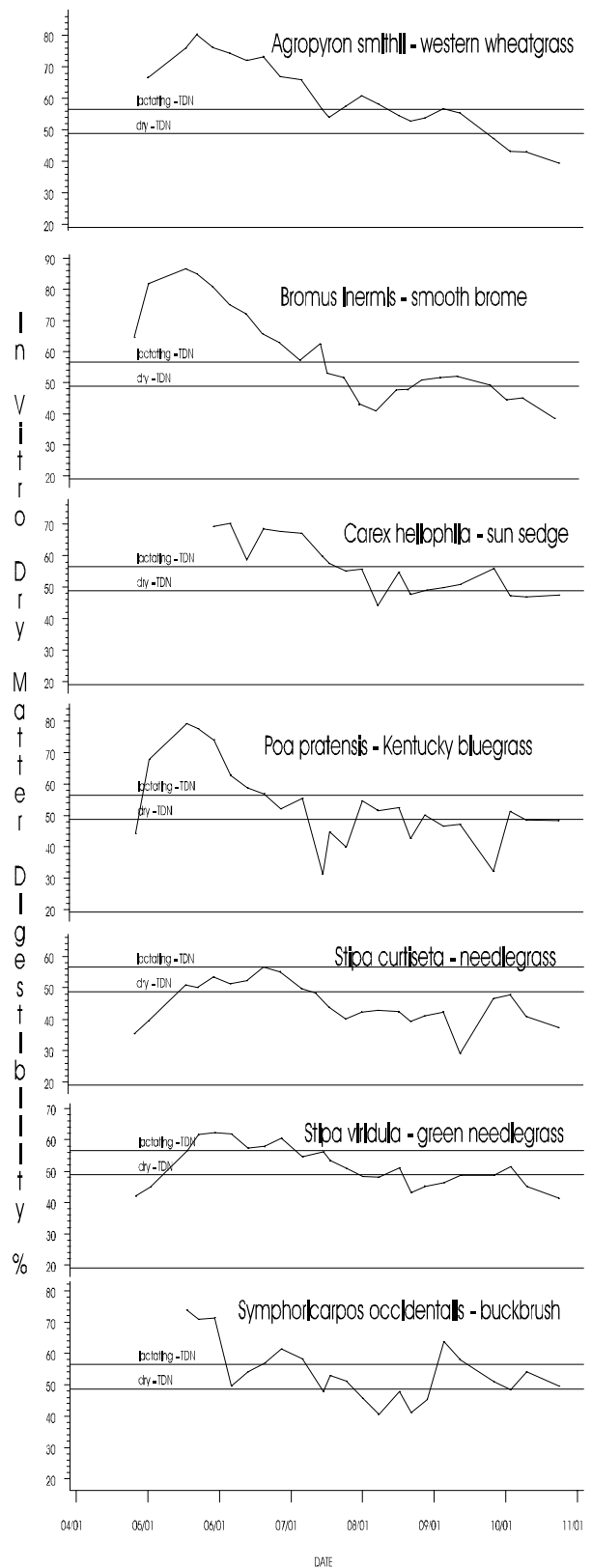
Figure 6. Seasonal changes for 1995 in the in vitro dry matter digestibility of the most abundant plant species on the grazing intensity trial. Reference lines indicate the total digestible nutrient requirement of a 1,000 lb lactating cow, average milkability (56.6%), and a 1,000 lb dry cow, middle third of pregnancy (48.8%) (NRC 1984).
