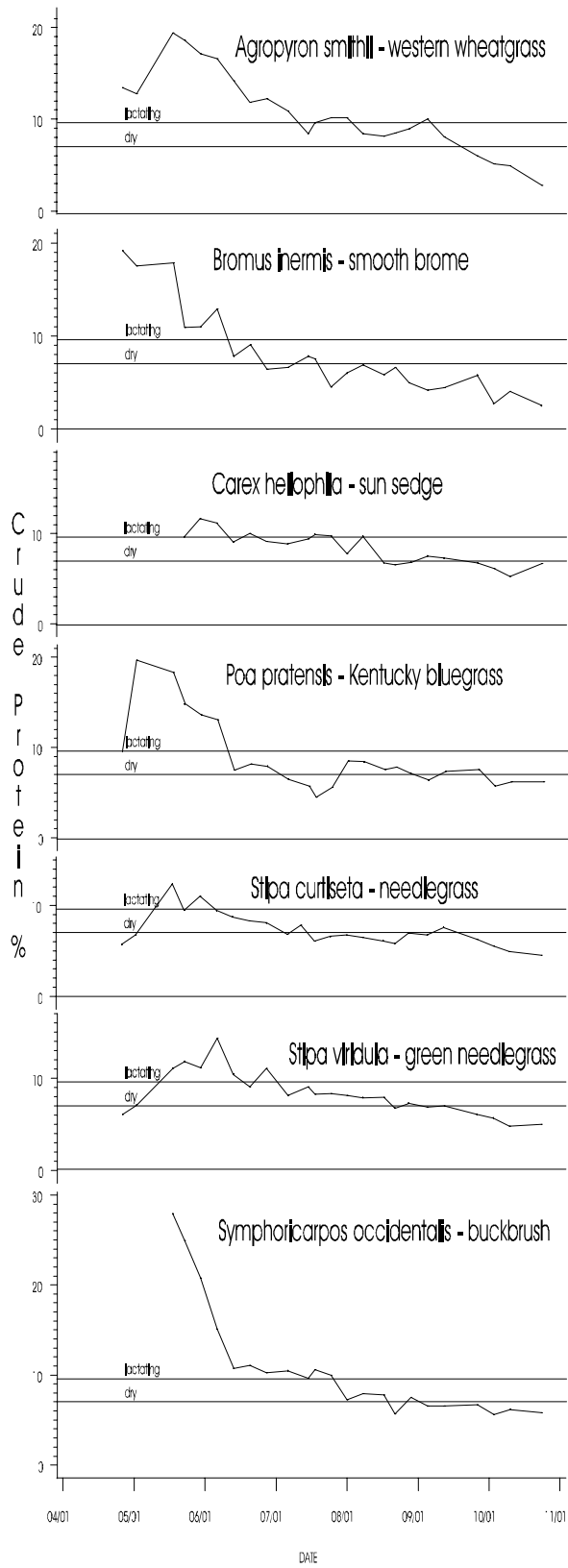
Figure 5. Seasonal changes for 1995 in crude protein content of the most abundant plant species on the grazing intensity trial. Reference lines indicate the crude protein requirement of a 1,000 lb lactating cow, average milkability (9.6%), and a 1,000 lb dry cow, middle third of pregnancy (7.0%) (NRC 1984).
