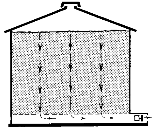
Figure 3. Aeration in grain equalizes the temperature and prevents serious moisture migration from occurring.
