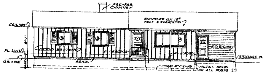
FRONT ELEVATION SCALE 1/8"=1'-0"
