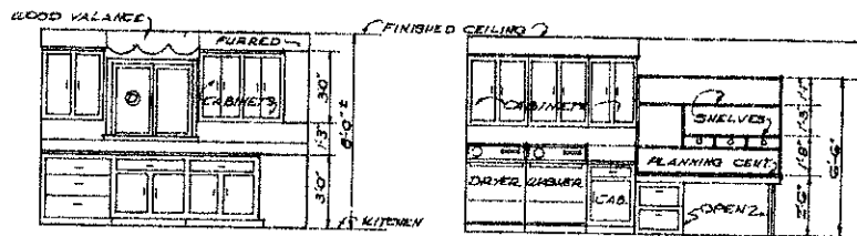
ELEVATION 'A' ELEVATION 'B' KITCHEN & LAUNDRY DETAILS SCALE 1/4"=1'-0"
