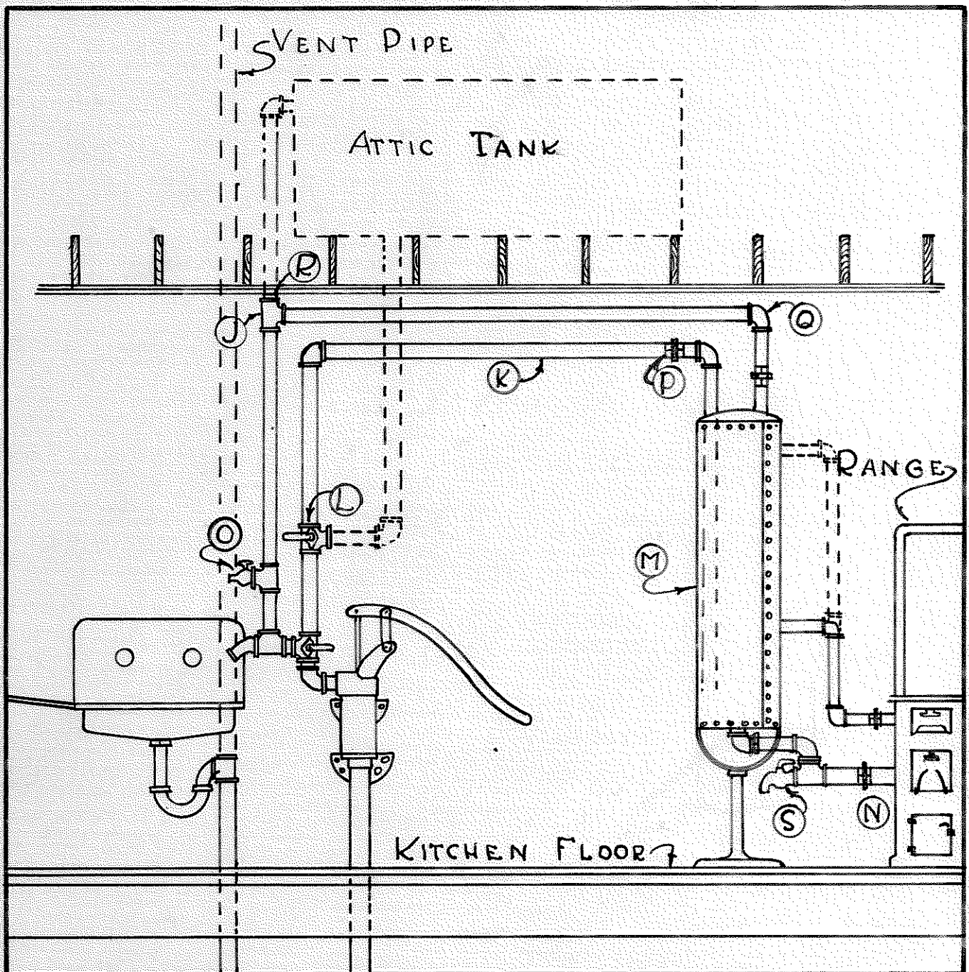
THE KITCHEN FORCE PUMP & RANGE BOILER PLAN NO. ND. 8533-1-11
