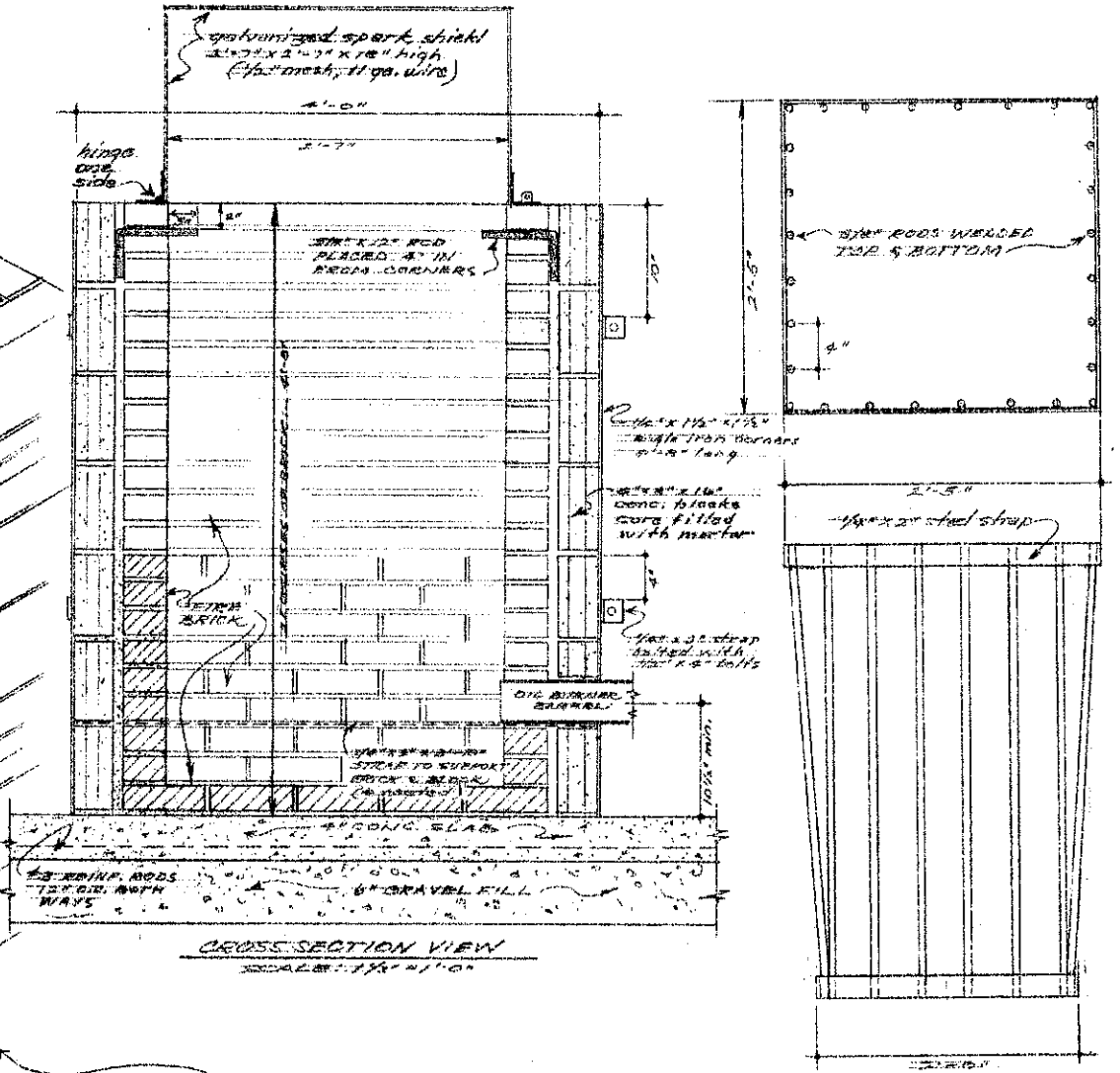
BASKET DETAILS
