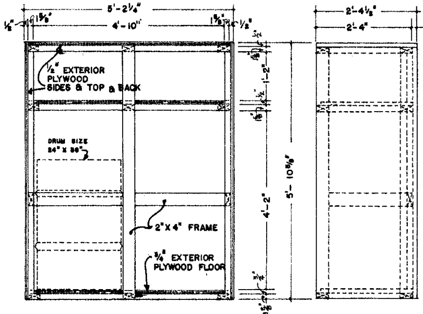
FRONT VIEW (DOORS NOT SHOWN)
