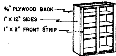
FRAMING PERSPECTIVE
