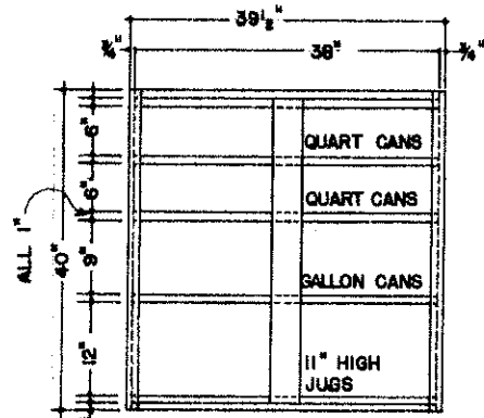
FRONT VIEW (WITHOUT DOORS)
