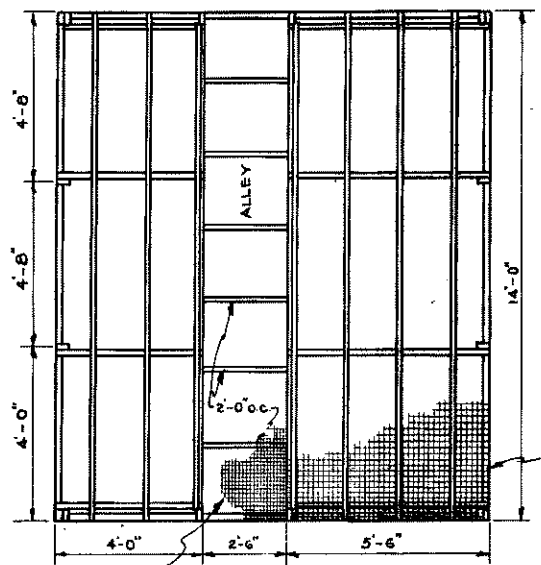
PLAN SCALE 3/8" = 1'-0"
