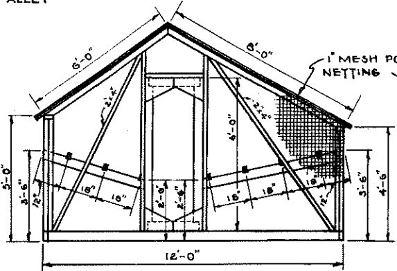
END VIEW SCALE 3/8" = 1'-0"
