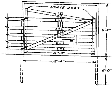
TYPICAL GATE
