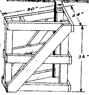
BLOCKING GATE
