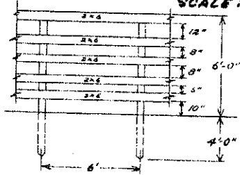
TYPICAL LINE FENCE
