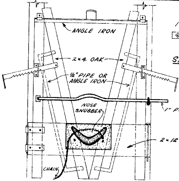
HEAD GATE DETAIL
