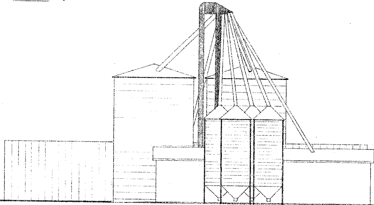
EAST ELEV. 1/8" = 1'-0"
