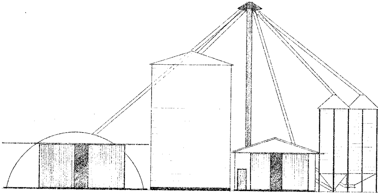
SOUTH ELEV. 1/8" = 1'-0"
