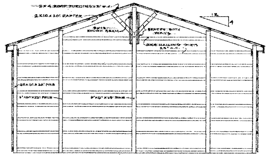
VIEW 11 CROSS SECTION OF END WALL
