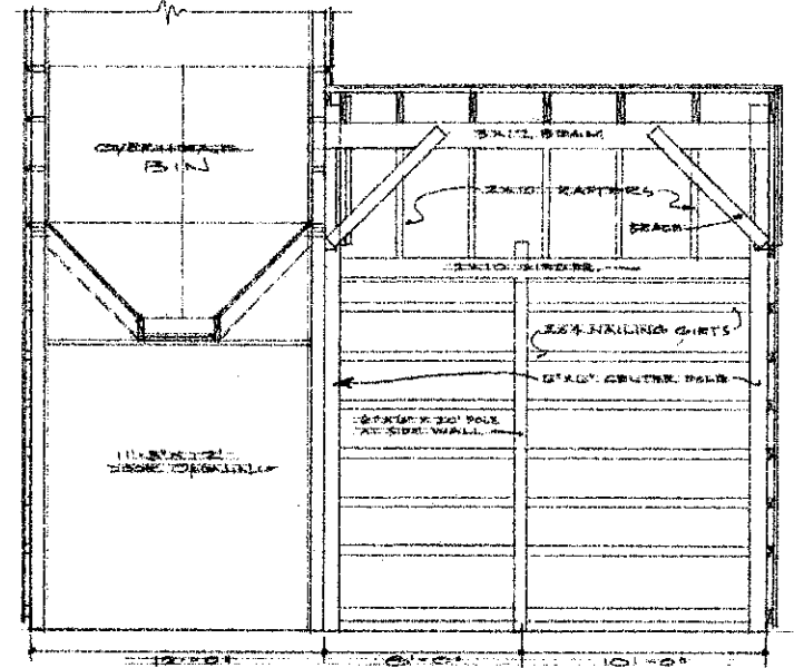
VIEW 10 CROSS SECTION OF BIN AND WORK AREA.
