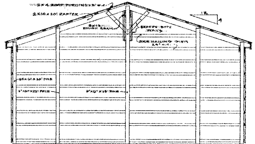
VIEW 9 CROSS SECTION OF END WALL
