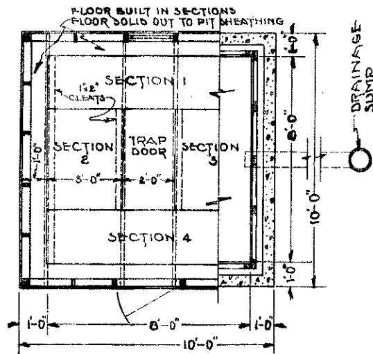
FLOOR PLAN WITH PART PIT PLAN SCALE: \frac{3}{8} = 1'-0"
