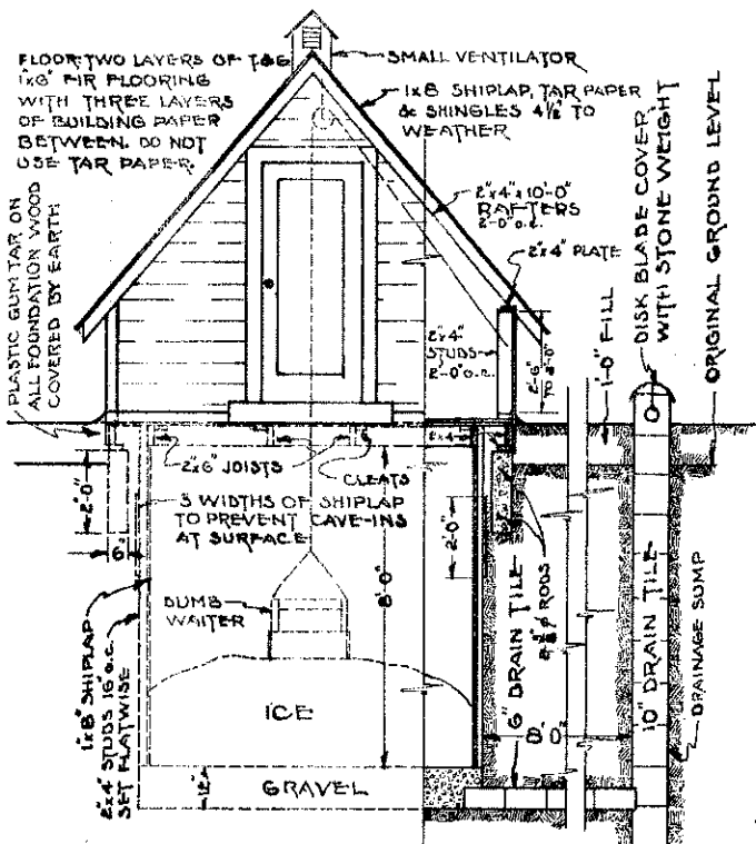
FRONT VIEW WITH PART SECTION SCALE: \frac{3}{8} = 1'-0"
