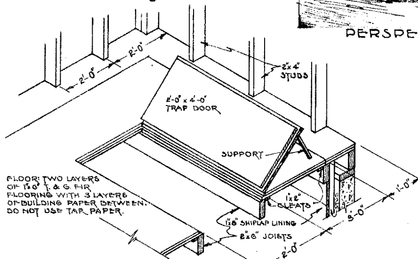
DETAIL OF FLOOR CONSTRUCTION SCALE: NONE
