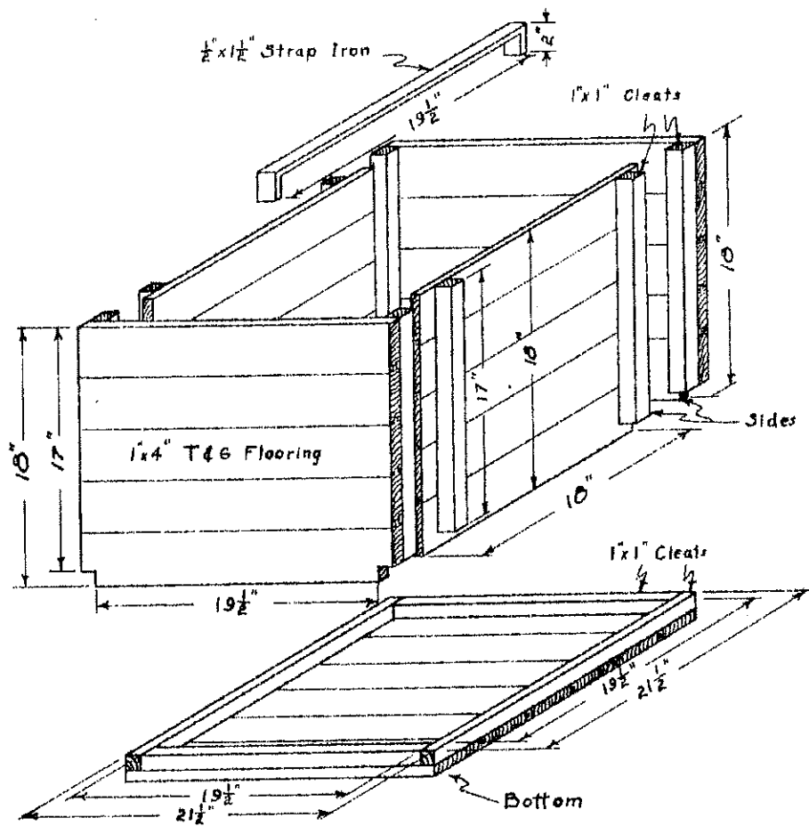
EXPERIMENTAL WOODEN ICE MOLD Mold sides held together at bottom by 1"x1" cleats nailed to bottom and at top by strap iron hook and outward pressure of water.
