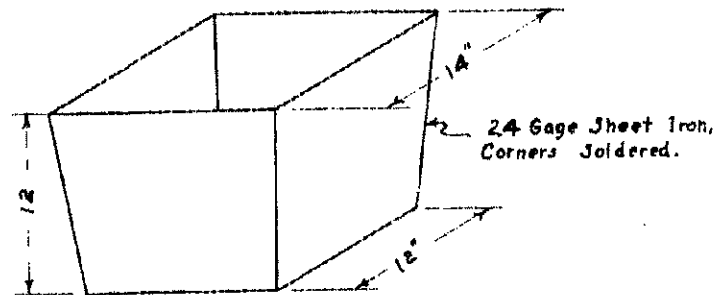
EXPERIMENTAL METAL ICE MOLD
