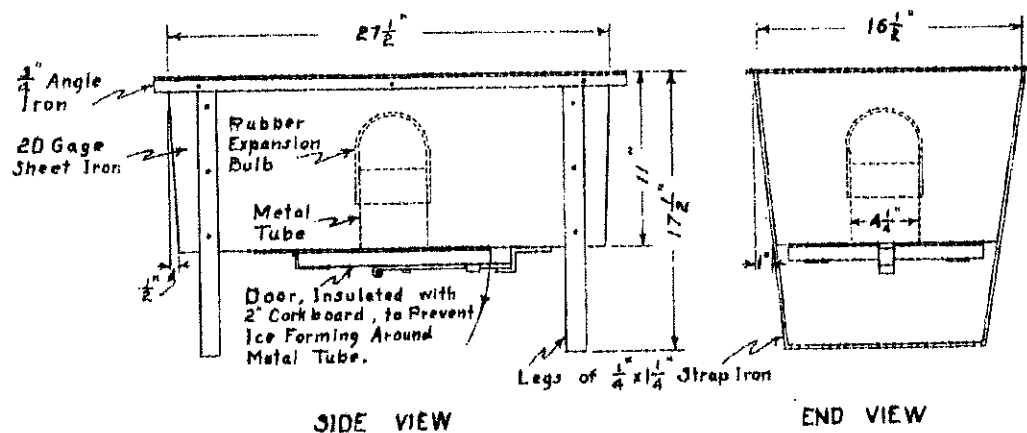
LATHAM'S ICE MOLD As water freezes over and expands, rubber expansion bulb collapses downward into metal tube.
