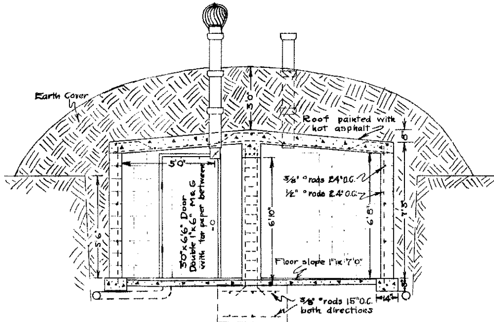
SECTION AT BB (Sheet 1)
