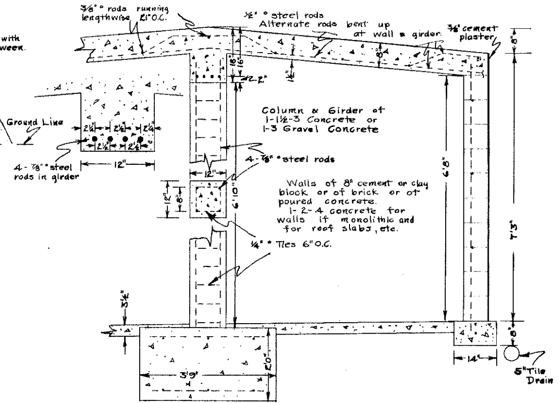
DETAIL SECTION Scale 3/4" = 1'0"
