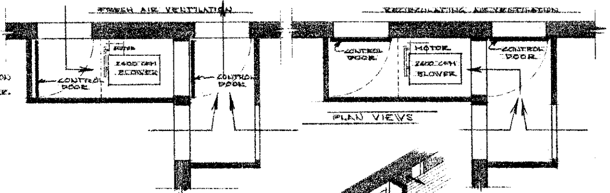
VENTILATION SYSTEM SCALE - 3/8" = 1'-0"
