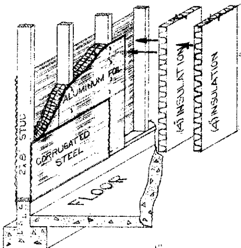
WALL INSULATION VIEW
