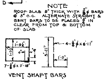
REINFORCING IN ROOF SLAB
