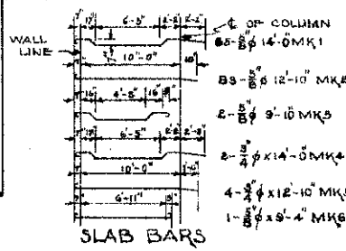
REINFORCING IN ROOF SLAB
