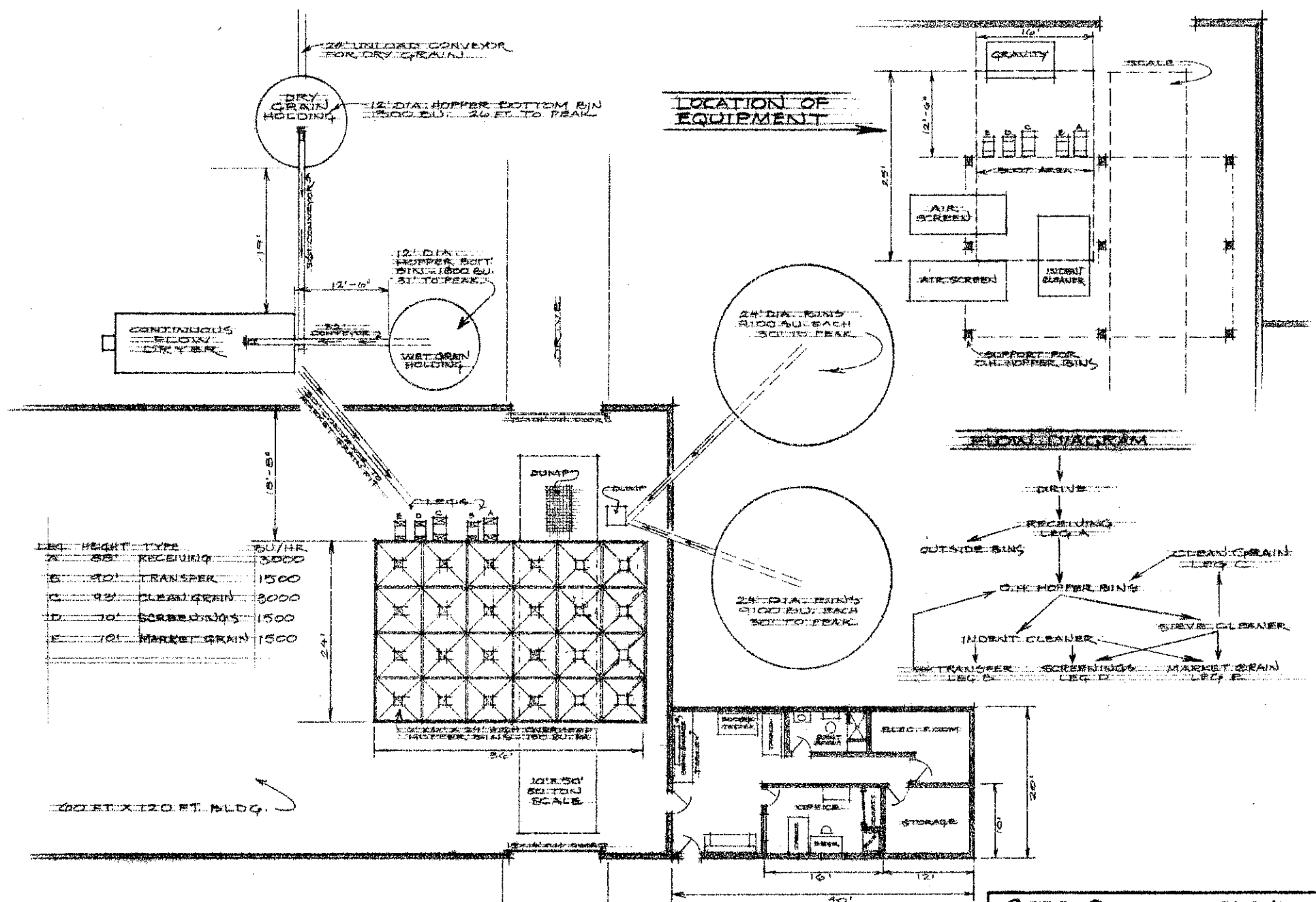
FLOOR PLAN
