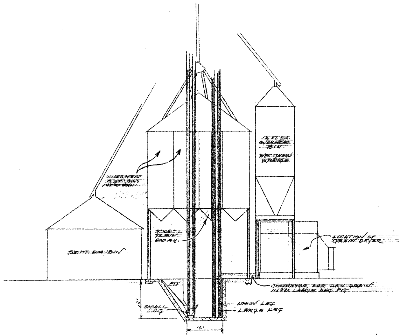
CROSS-SECTION VIEW B-B'
