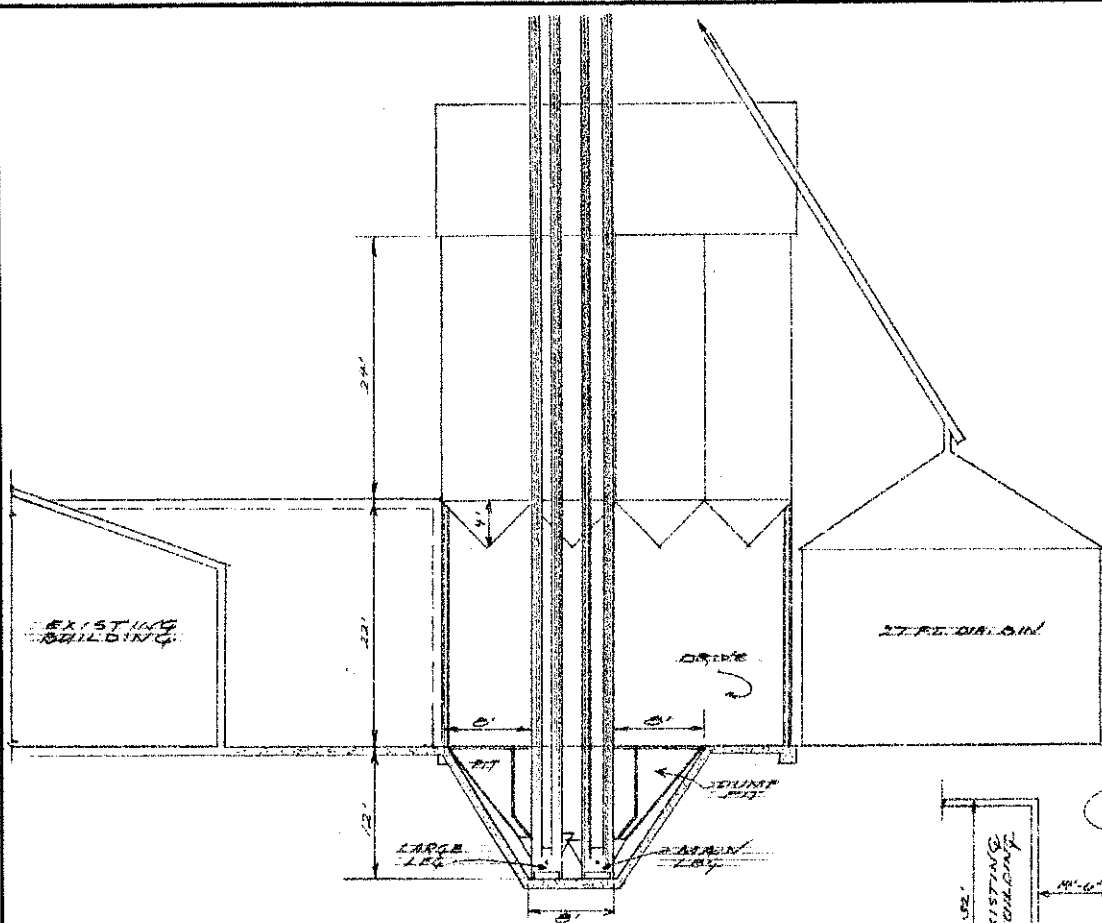
CROSS-SECTION VIEW A-A'
