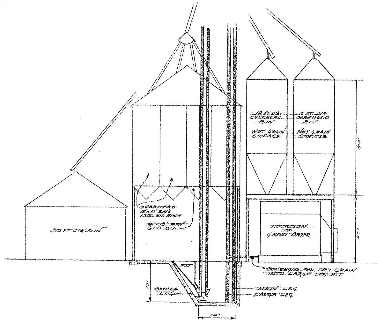
CROSS-SECTION VIEW B-B'
