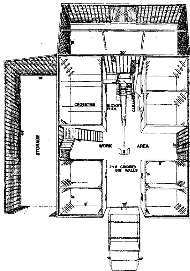
CUTAWAY VIEW
