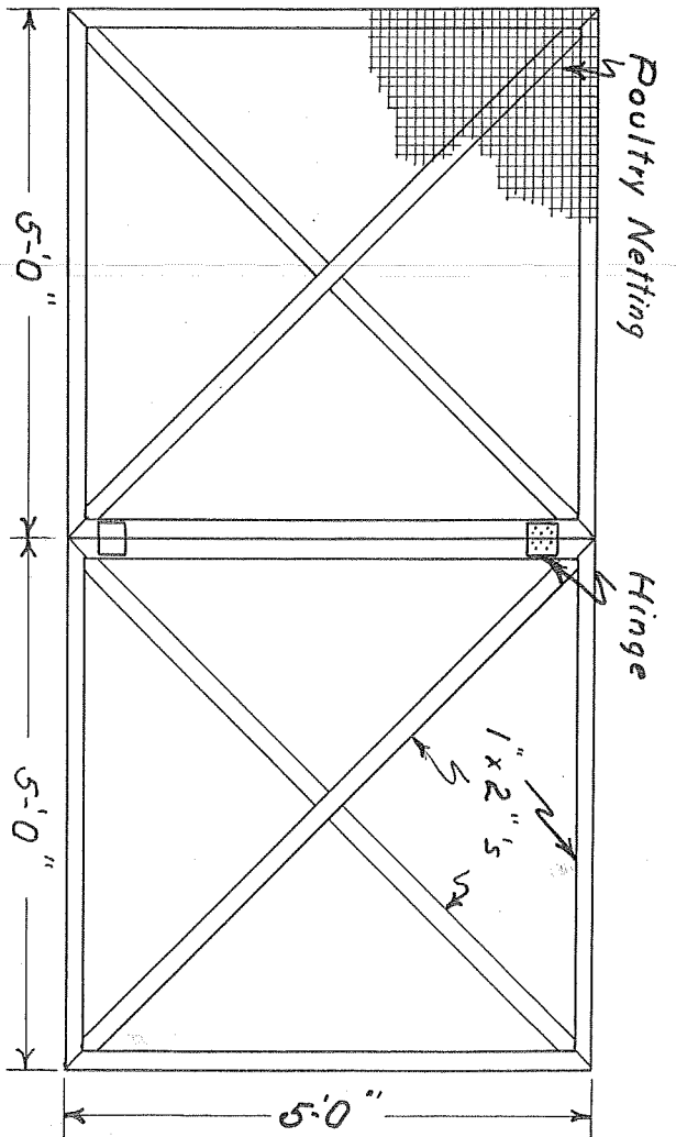
CATCHING FRAME - Scale: \frac{1}{2} " = 1'-0"
