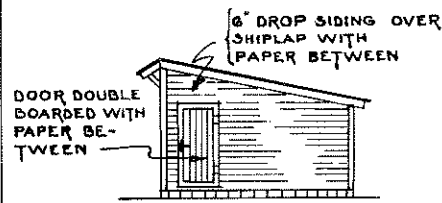
RIGHT END ELEVATION SCALE \frac{1}{2}''=1'-0''
