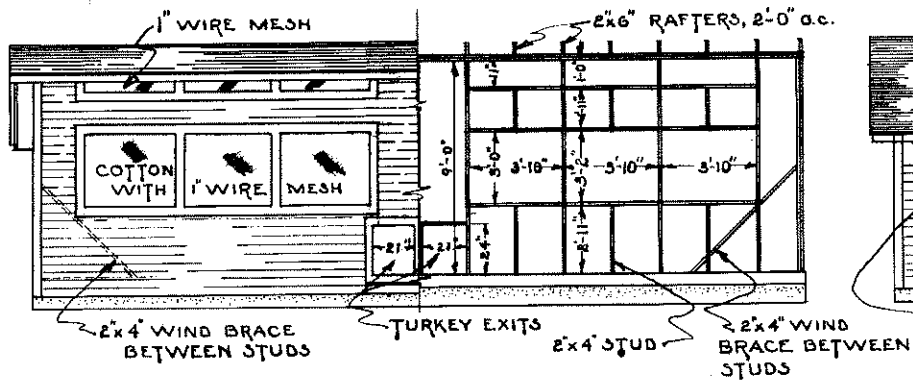
FRONT ELEVATION AND FRAMING SCALE \frac{1}{4}''=1'-0''
