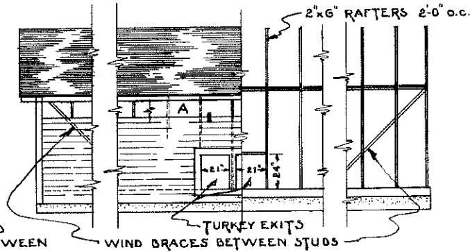
REAR ELEVATION AND FRAMING SCALE \frac{1}{4}''=1'-0''
