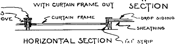
HORIZONTAL SECTION DETAIL OF MUSLIN CURTAIN SCALE \frac{3}{4}''=1'-0''
