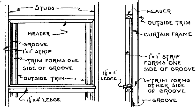
INSIDE VIEW WITH CURTAIN FRAME OUT VERTICAL SECTION
