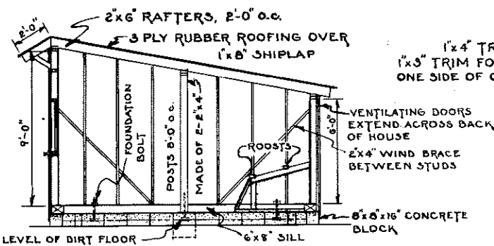
SECTION THRU WINDOW SCALE \frac{1}{4}''=1'-0''
