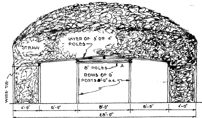
SECTION OF STRAW CATTLE SHED SCALE \frac{1}{16} = 1'-0"
