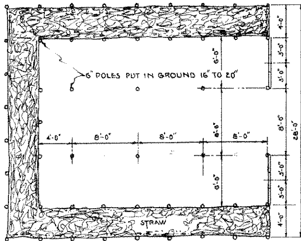
PLAN SCALE \frac{1}{16} = 1'-0"
