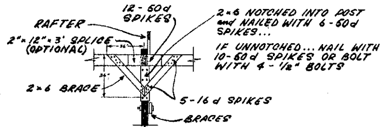
DETAIL OF BRACES AT PURLIN
