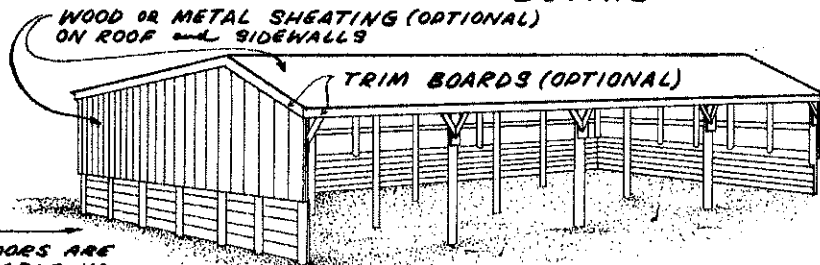
PERSPECTIVE
