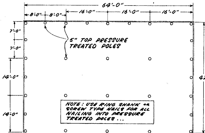
FLOOR PLAN
