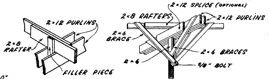
RAFTER TIE DETAIL
