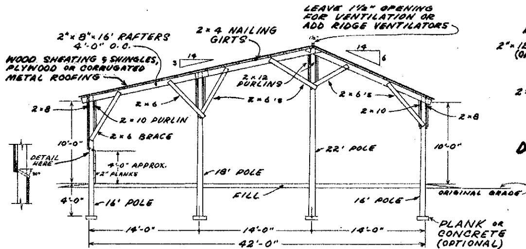
CROSS SECTION
