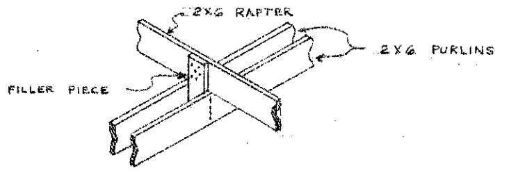
RAFTER TIE
