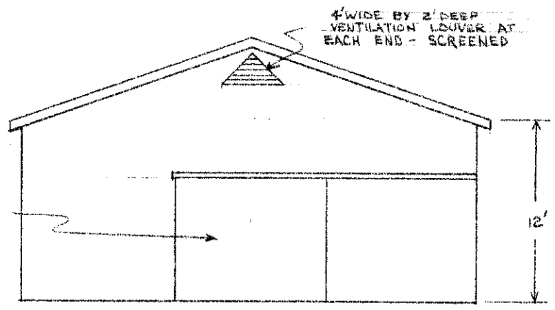
END VIEW
