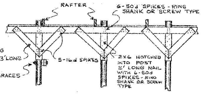
BRACES AT PURLIN
