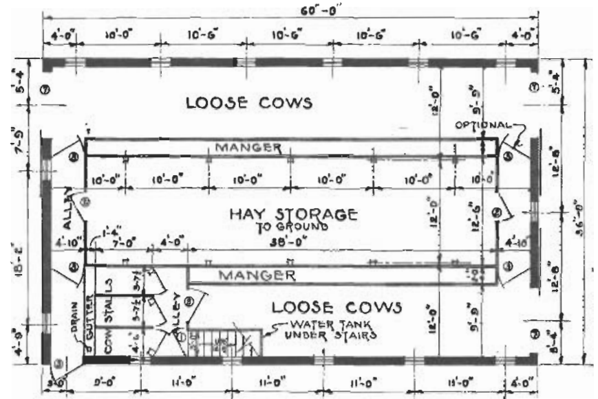
PLAN 6 Scale \frac{1}{8}'' = 1'-0''
