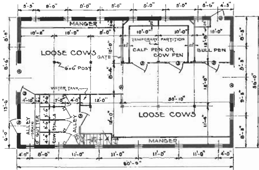
PLAN 7 Scale \frac{1}{8}'' = 1'-0''
