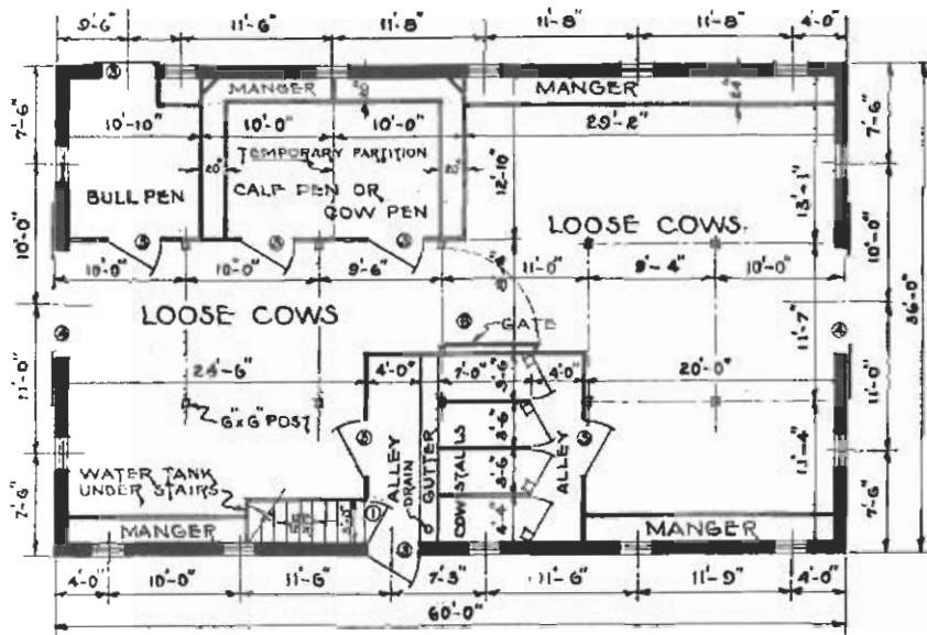
PLAN 5 Scale \frac{1}{8}'' = 1'-0''
