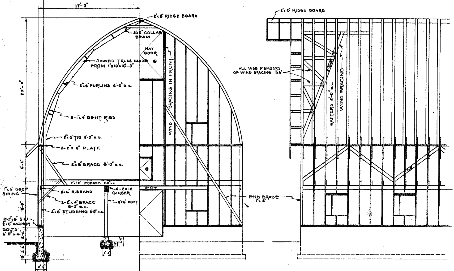
HALF CROSS SECTION
