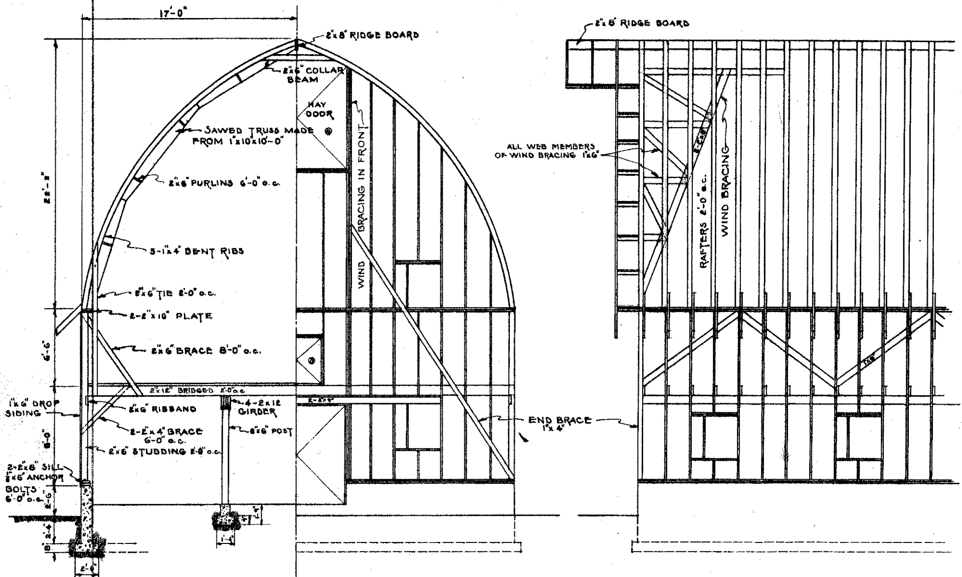
HALF CROSS SECTION
