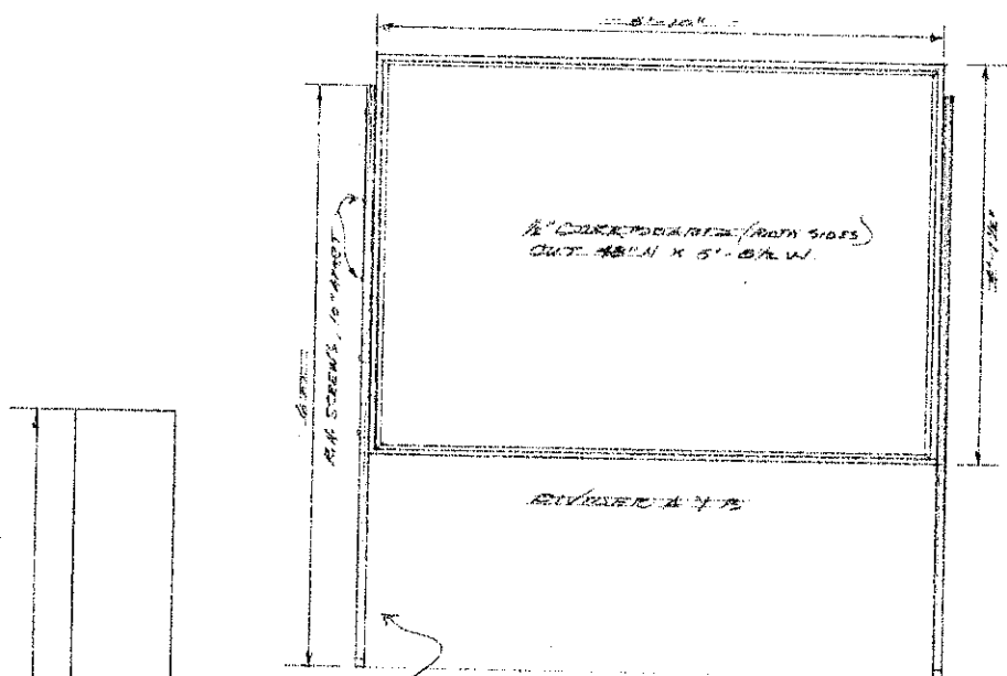
ELEVATION VIEW TYPICAL DIVIDER (FRONT) (NEED TWO THIS SIZE)
