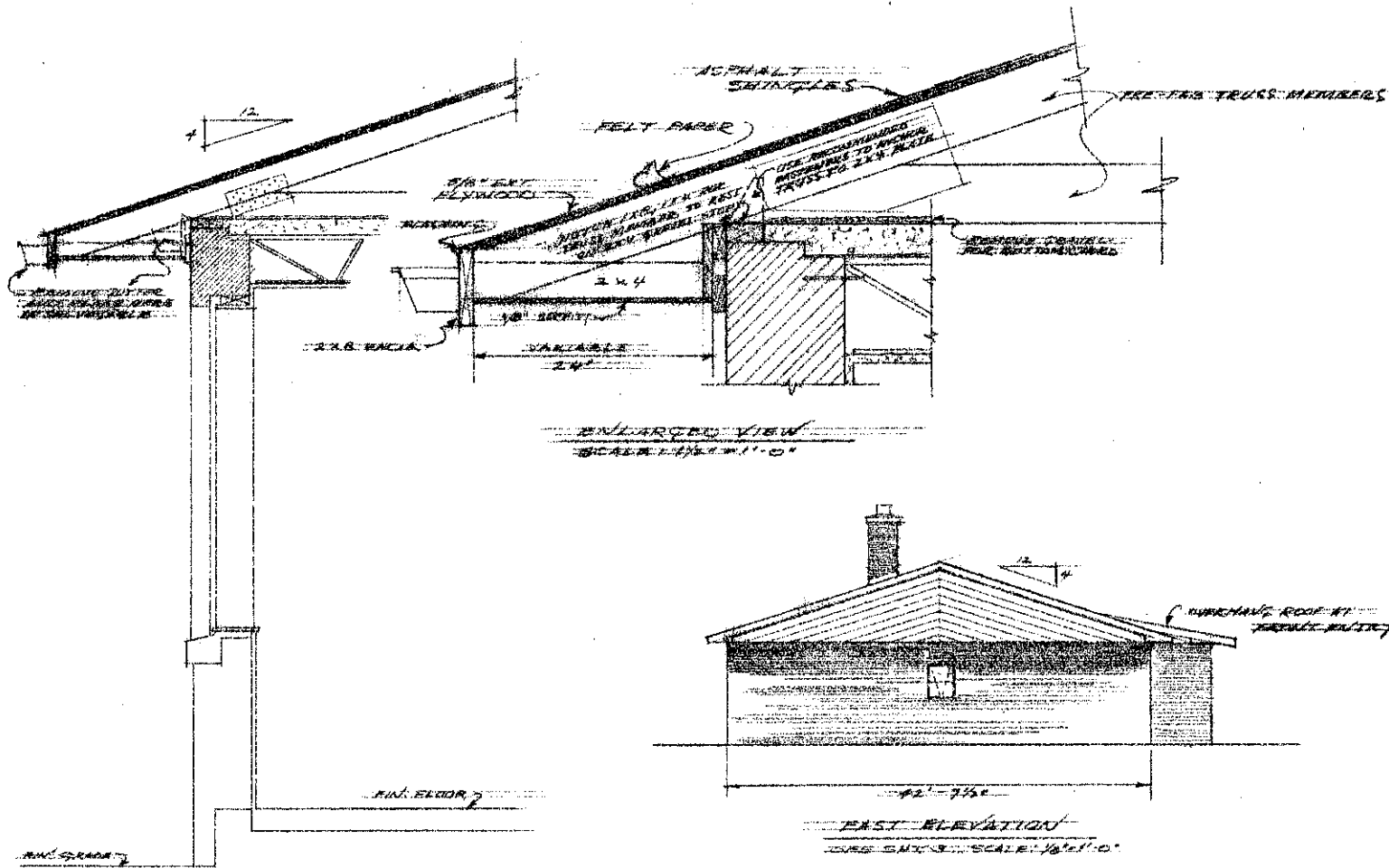
CROSS SECTIONAL VIEW AS SHOWN ON SHEET 6 SCALE 1/4" = 1'-0"
