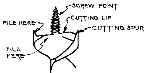
FIG. 6 AUGER BIT
